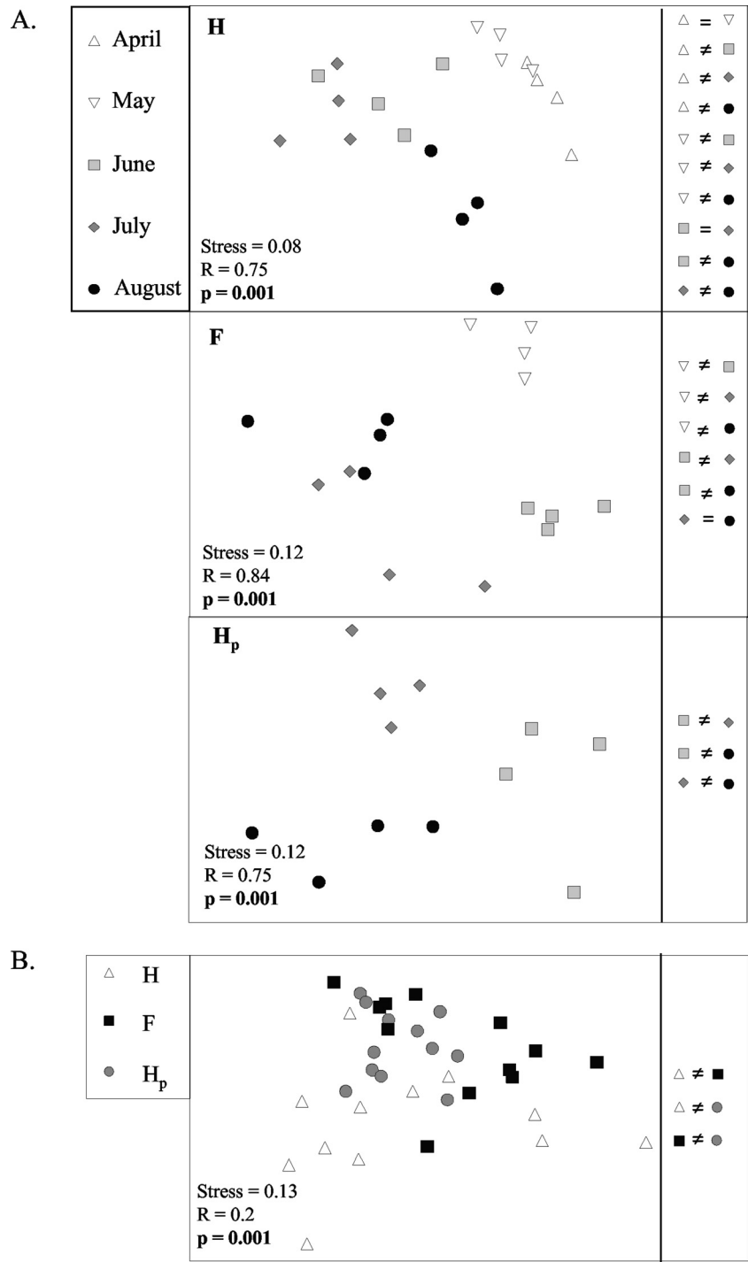
FIG. 1. MDS representation of the structure of the nirK denitrifier community (assessed by DGGE analysis of nirK genes) on different sampling dates for three spatial locations, H, Hp, and F, in soil under potato cultivation (A) and at different row locations across the sampling dates (from June to August) (B). The similarities or differences in community structures are indicated. See Tables 1 and 2 for results of ANOSIM.
